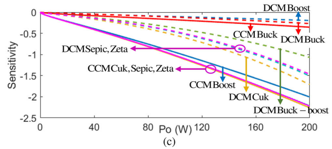
FIGURE 19 Sensitivity comparison of NIDC-DC converters with respect to P_o at t = 0.6 \times 10^6 h: Components sensitivities in (a) DCM and (b) CCM operating modes; (c) Converters' overall sensitivities
