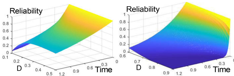
FIGURE 7 Reliability performance of the Cuk converter with respect to D and t ( \text{h} \times 10^6 ): (a) DCM; (b) CCM
