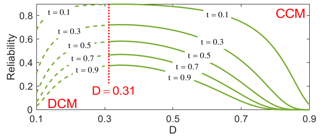
FIGURE 8 Reliability performance of the Buck-Boost converter with respect to D in different t ( \text{h} \times 10^6 )
