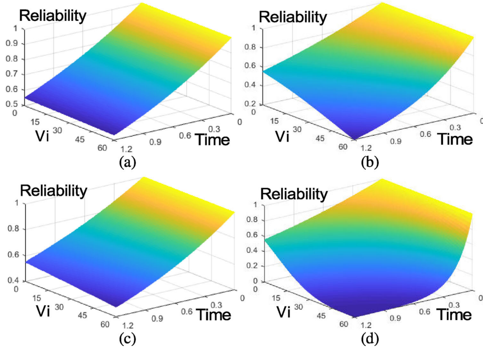
FIGURE 12 Reliability performance of the NIDC-DC converter topologies with respect to V_i (V) and t ( h \times 10^6 ): (a) DCM Buck; (b) DCM Boost; (c) CCM Buck; and (d) CCM Boost
