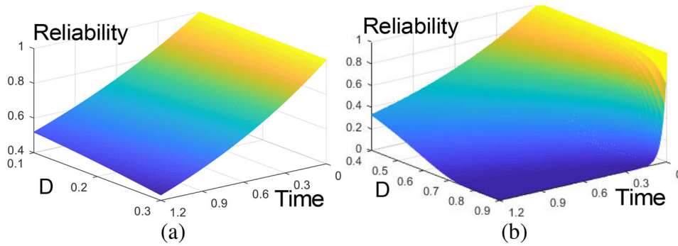
FIGURE 6 Reliability performance of the Boost converter with respect to D and t ( \text{h} \times 10^6 ): (a) DCM; (b) CCM
